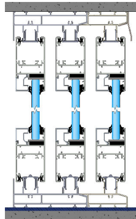
Corte Vertical
